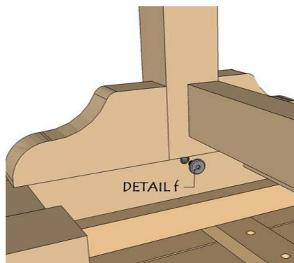
DETAIL f
